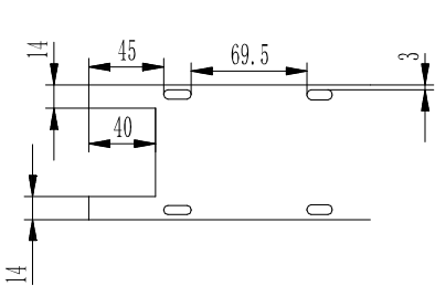
DETAIL G SCALE 1:5
