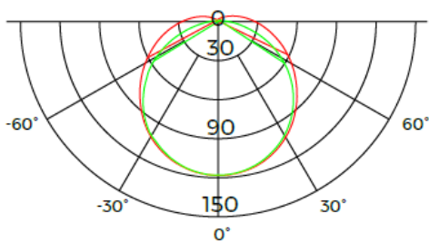
PHOTOMETRIC OF 1M LUMINAIRE (D6120-24V-8mm)
