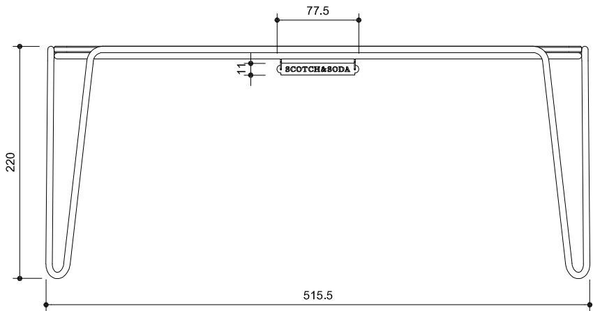
FRONT VIEW 正视图 SCALE: 1:5
