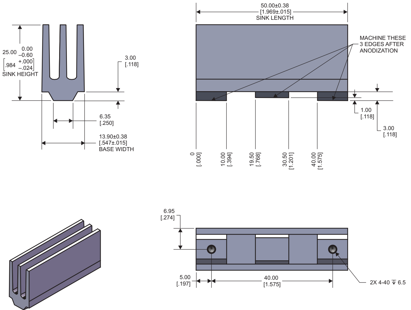
Figure 35. EVM Heatsink
