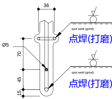
DETAIL D (1:5)
