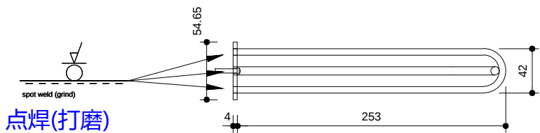
DETAIL A (1:5) 细节A
