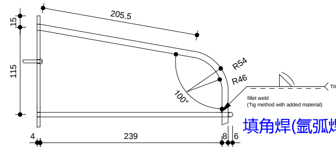
DETAIL B (1:5)
