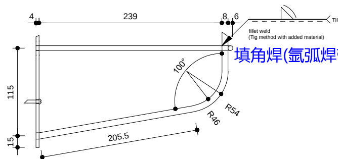
DETAIL C (1:5)
