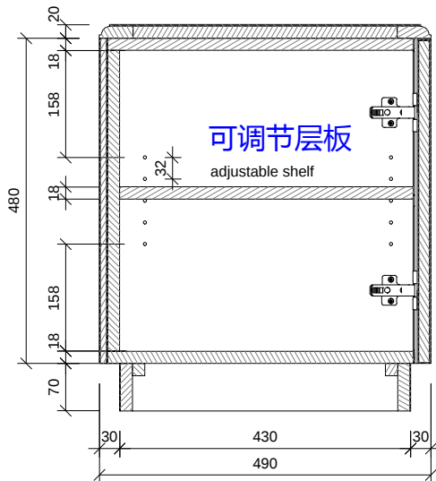
SECTION E (1:10) 截面E
