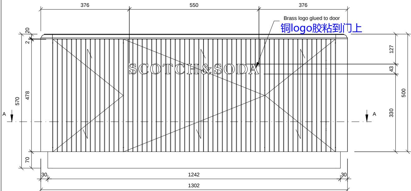
FRONT VIEW SCALE 1:10
