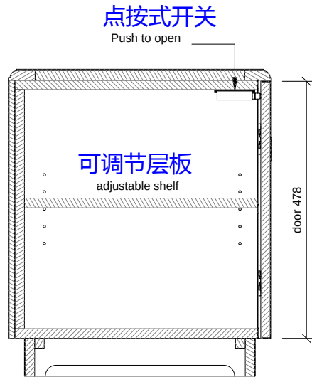
SECTION R (1:10) 截面R
