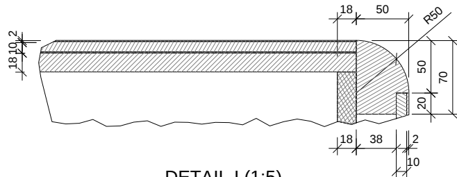
DETAIL I (1:5) 细节I
