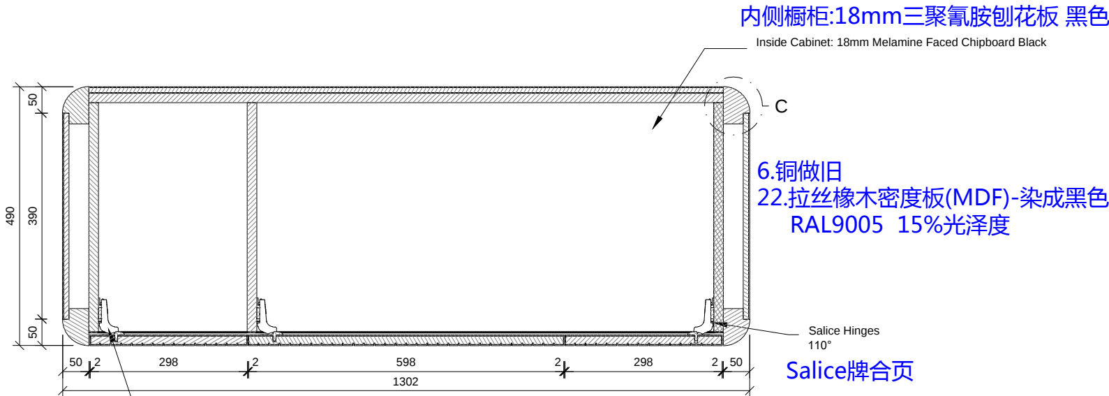
SECTION A (1:10)
