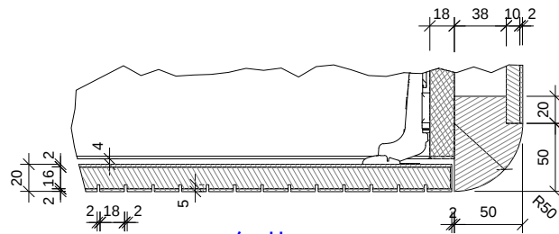
细节H DETAIL H (1:5)
