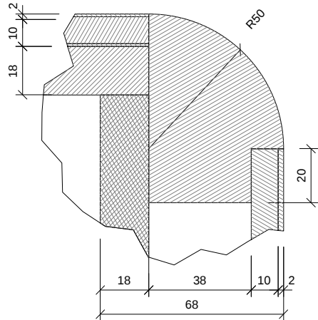
DETAIL C (1:2)
