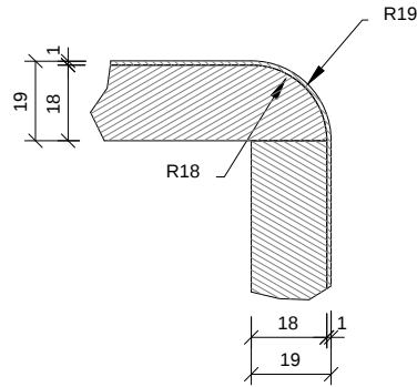
DETAIL G (1:2) G细节
