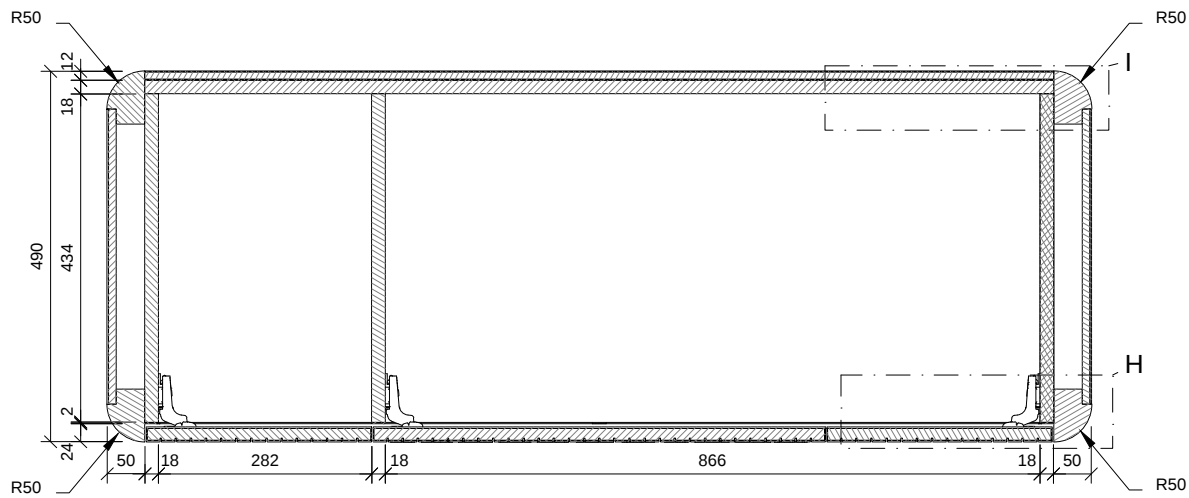
SECTION D (1:10) 截面D 门298 门598 门298
