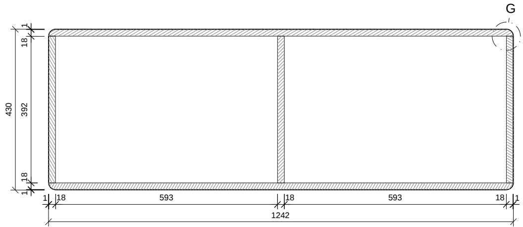
SECTION F (1:10) 截面F
