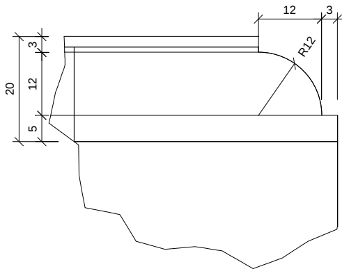
DETAIL B (1:1)
