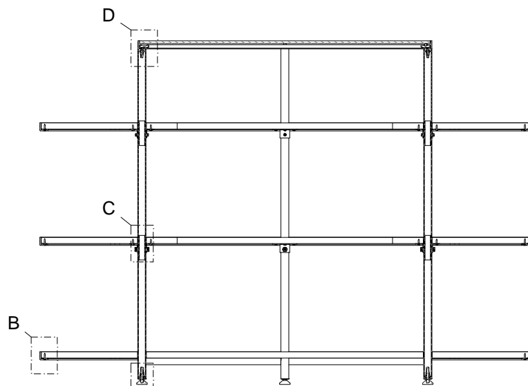
截面A SECTION A (1:16)
