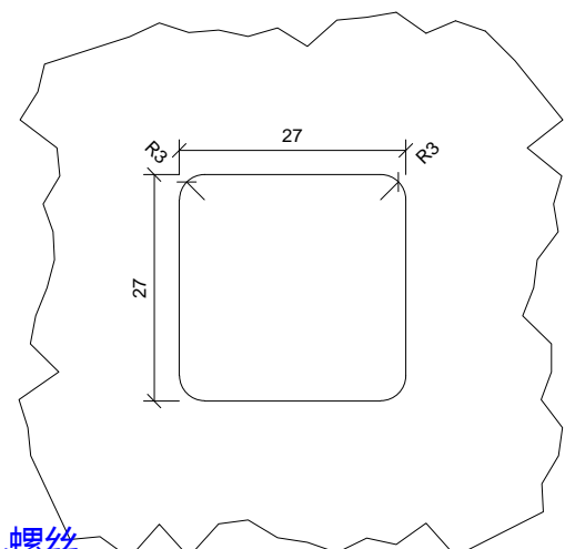
DETAIL I (1:1) 细节I
