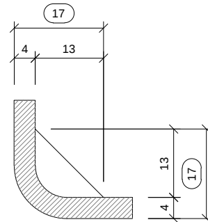
SECTION F (1:1) 截面F
