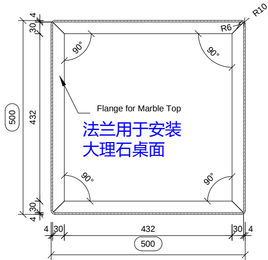
SECTION D (1:10) 截面D
