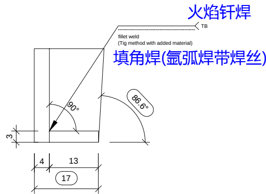
DETAIL C (1:1) 细节C
