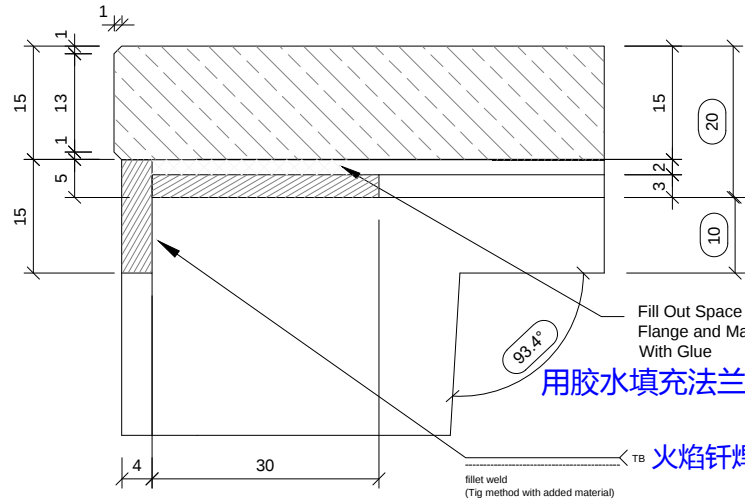
DETAIL B (1:1) 细节B
