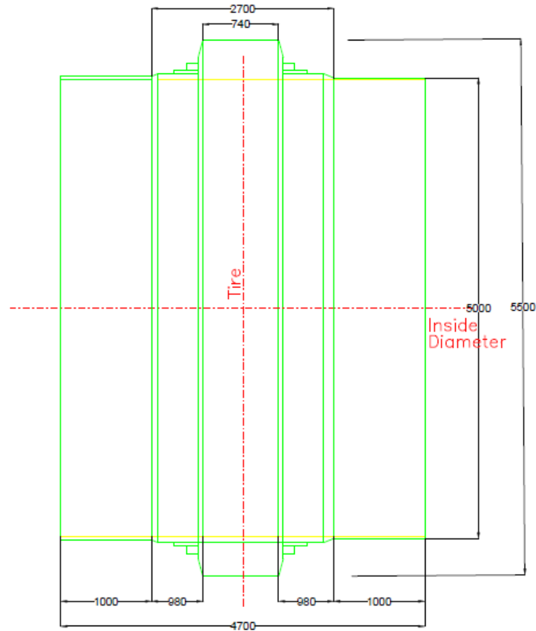
Kiln Tire 轮带
