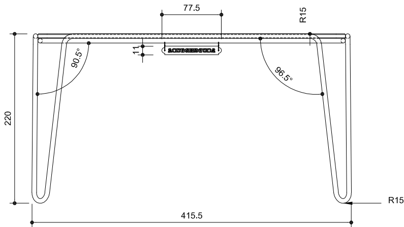
FRONT VIEW SCALE: 1:5 正视图
