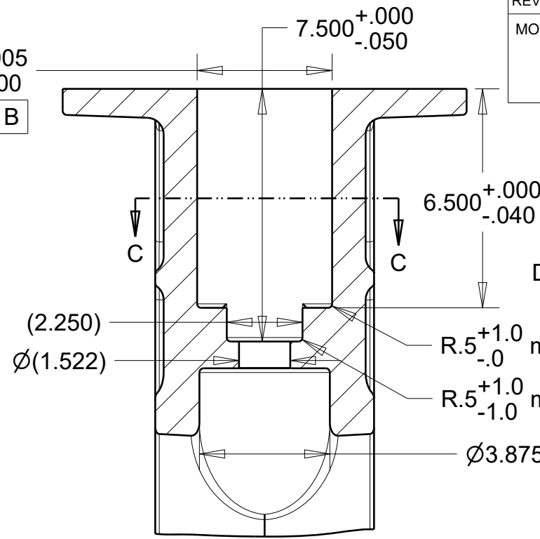
SECTION B-B SCALE 1/4
