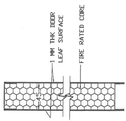
TYPICAL DOOR TOP BOTTOM DETAIL
