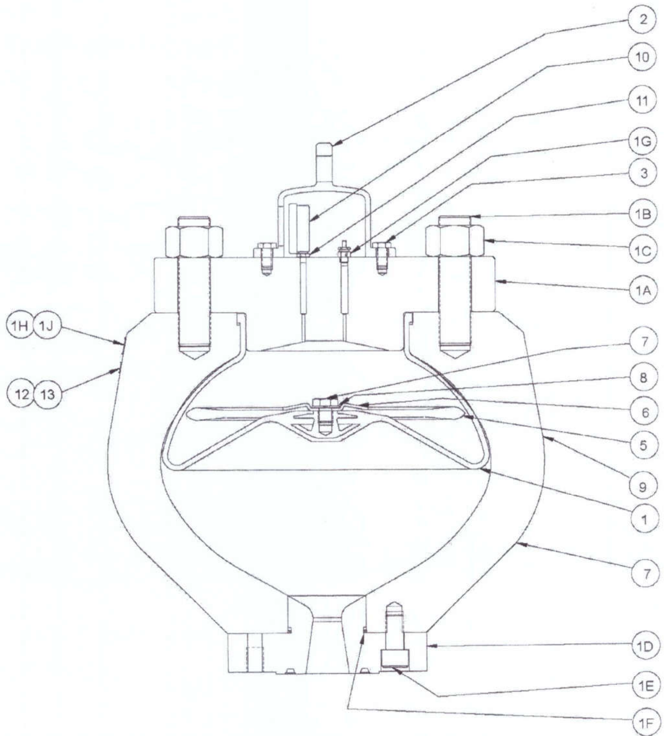
Figure 6-1. Typical K20-7500 Series Pulsation Dampener - Cutaway for Part Identification
